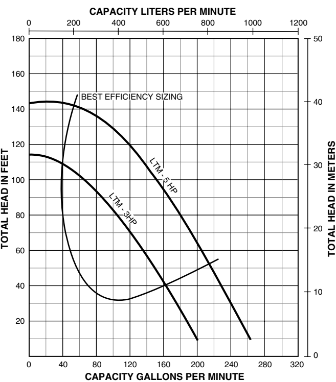
PUMP PERFORMANCE - LTM MEDIUM HEAD
